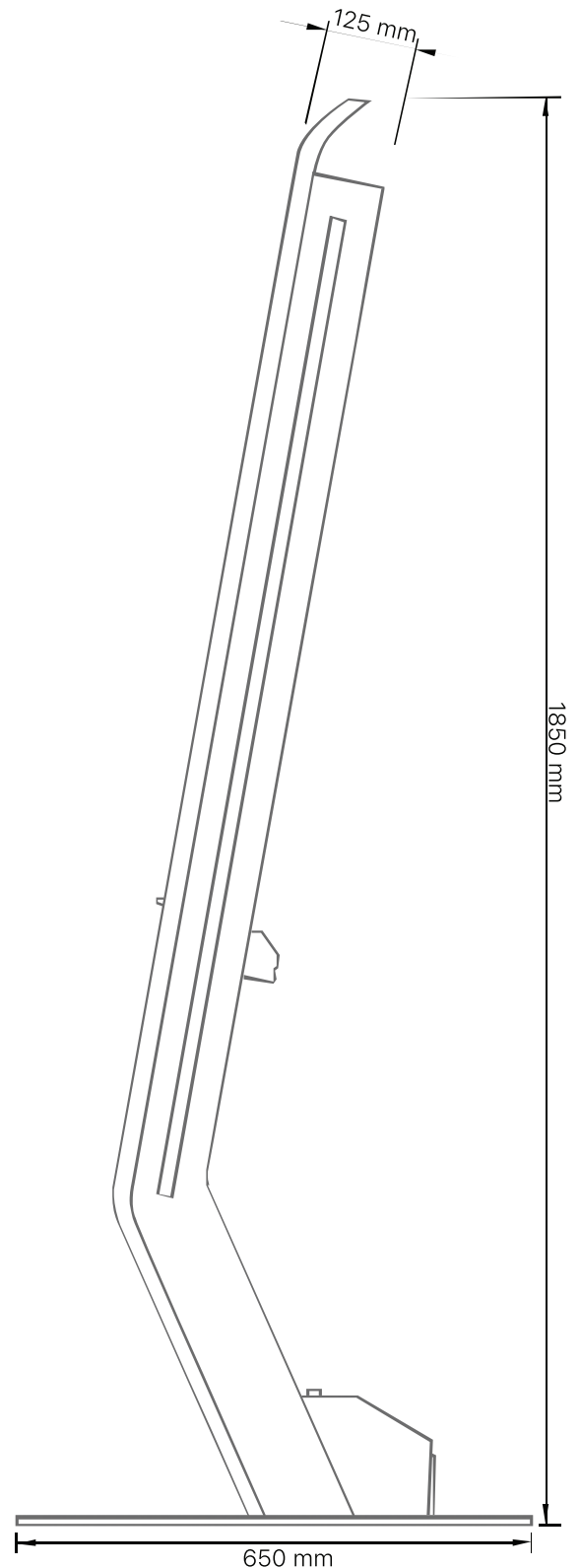
Side View
