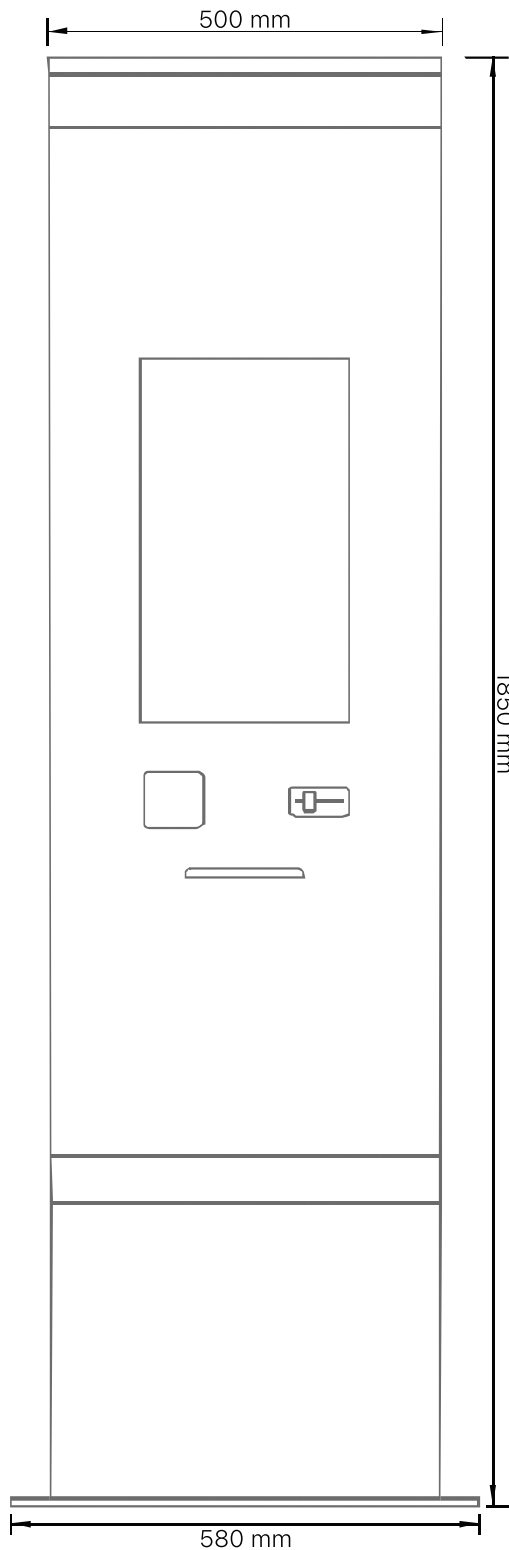
Front View
